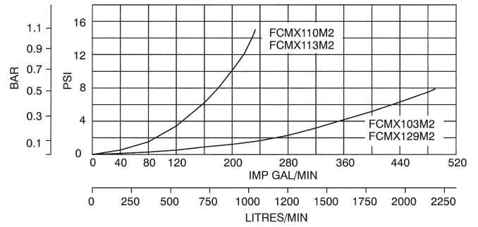
Pressure Loss Curves
