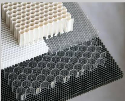
Honeycomb Laminar Air Flow Units
