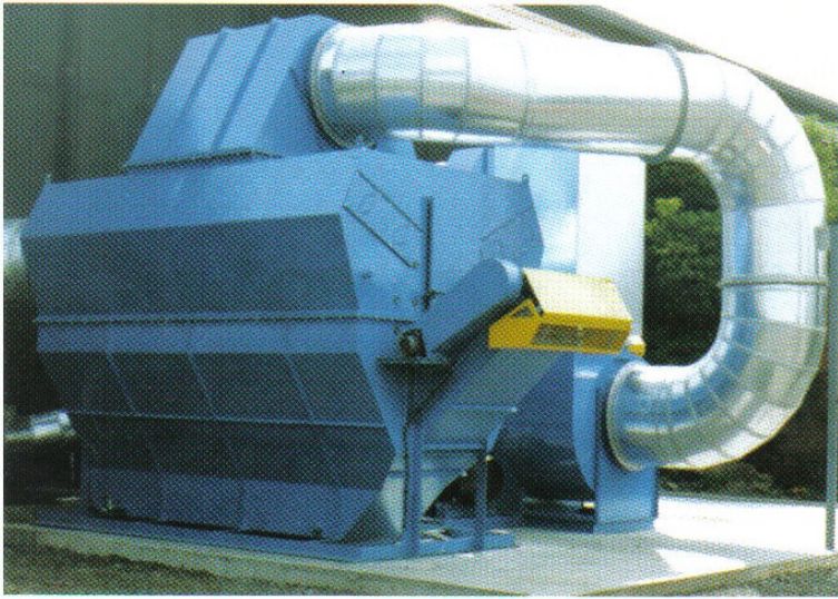
Hand/Auto De-sludge Wet Arrestors
