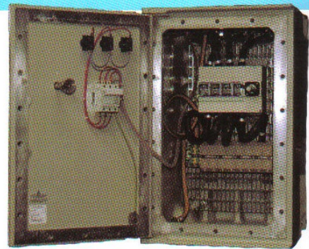
EExe PORTABLE TRANSFORMER UNITS & SPLITTER BOXES 400/240/110v INPUT SUPPLY 110/240V OUTPUTS
