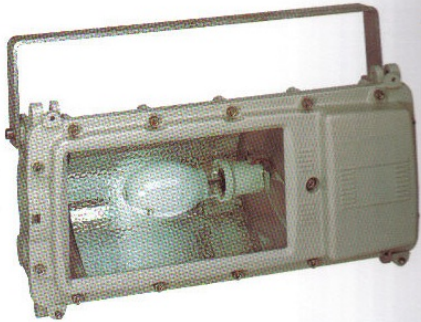
EExd WELLGLASS LUMINAIRES 70 - 200 WATT
