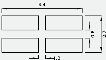
KPB-3025, KPBL-3025
