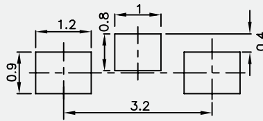
KPA-3210
