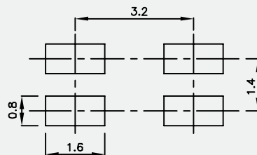
KPBD-3224
