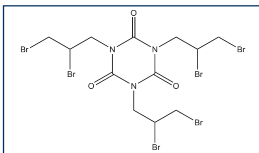
Tris(2,3-dibromopropyl)isocyanurate (T23BPIC)
