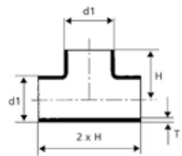
Equal tees with branch
