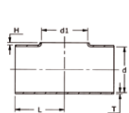
Pulled equal and reducing tees
