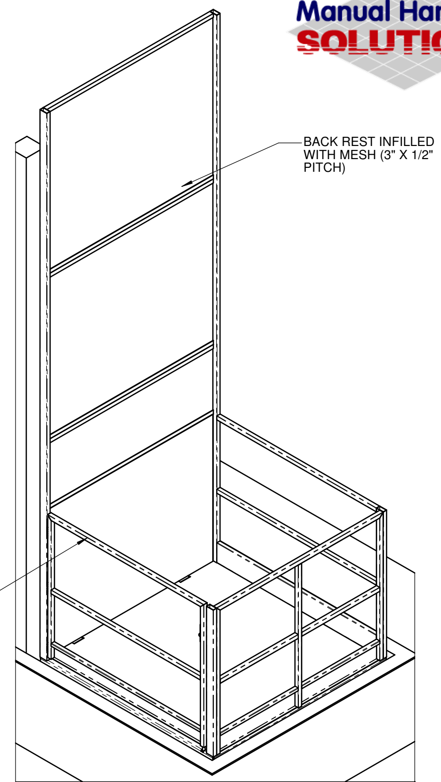
DETAIL A SCALE 2 : 45
