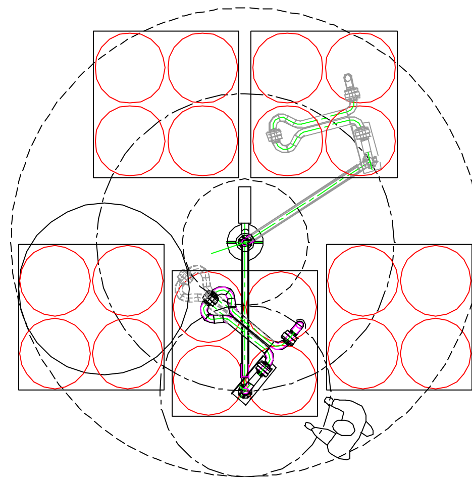
PLAN DETAIL SHOWING 360 DEGREE OPERATION
