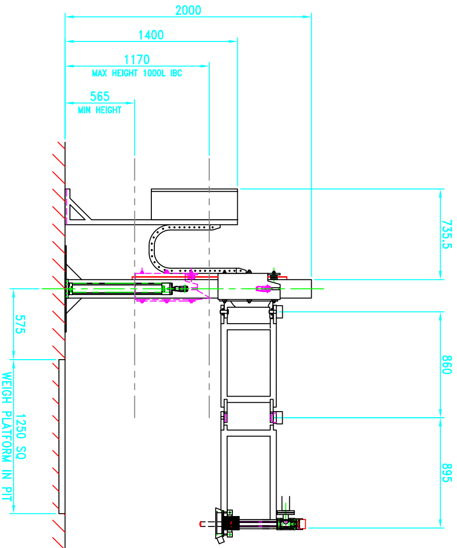
SIDE VIEW ON ARROW A
