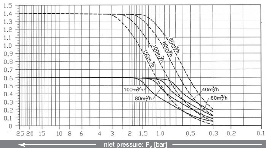
Dynamic expansion curve (1013 mbar / 14.7 psi, 0 °C / 32 °F)
