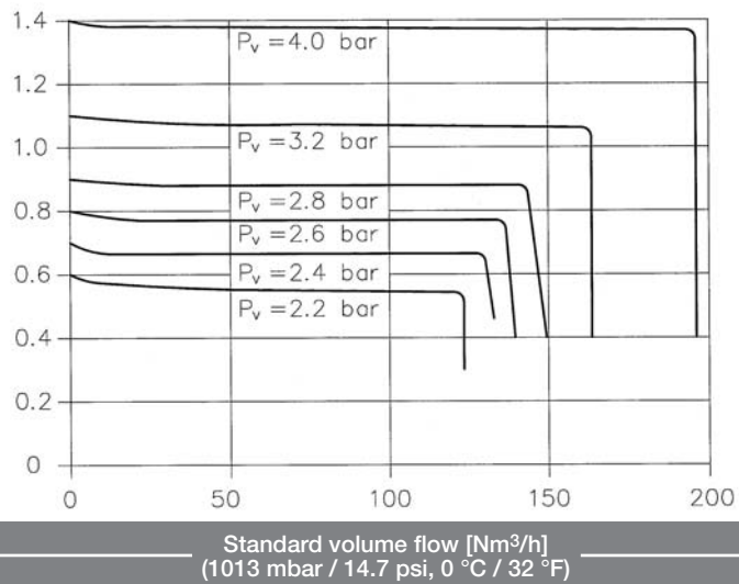
Dynamic expansion curve (1013 mbar / 14.7 psi, 0 °C / 32 °F)
