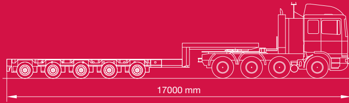
5 Axle Semi Low Loader
