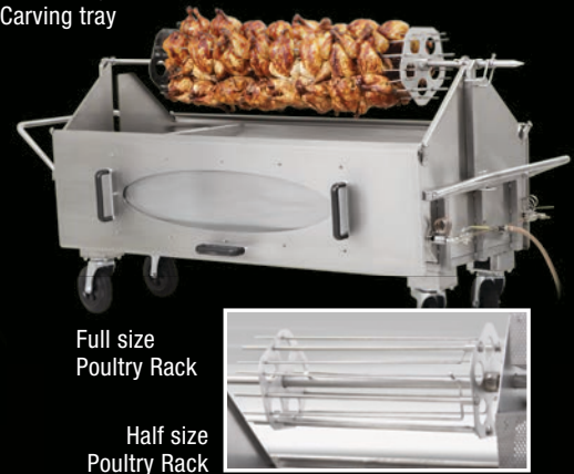
Spit Roast Machine with Motor, Spit Pole, Tools and Carving tray
