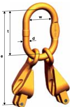
VXKW 2 Clevis master set
