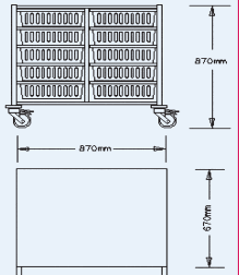
Plan View
