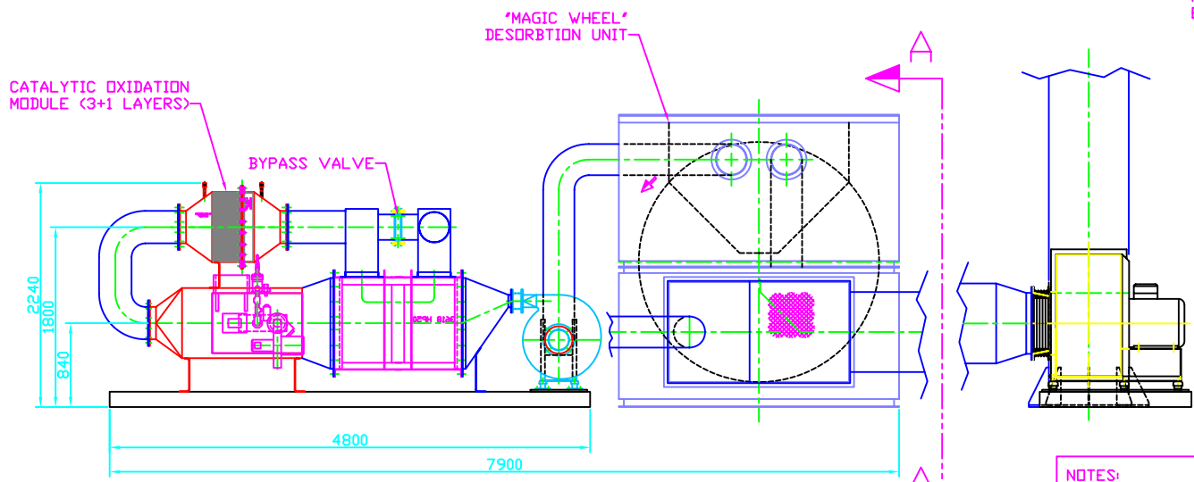
SECOND STAGE HEAT EXCHANGER AND ASSOCIATED DUCTS OMITTED FOR CLARITY
