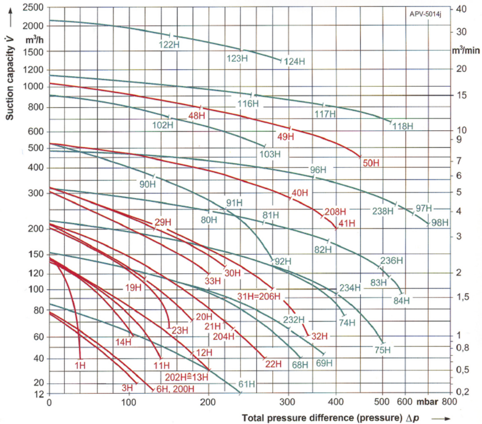
Selection diagram compressor operation
