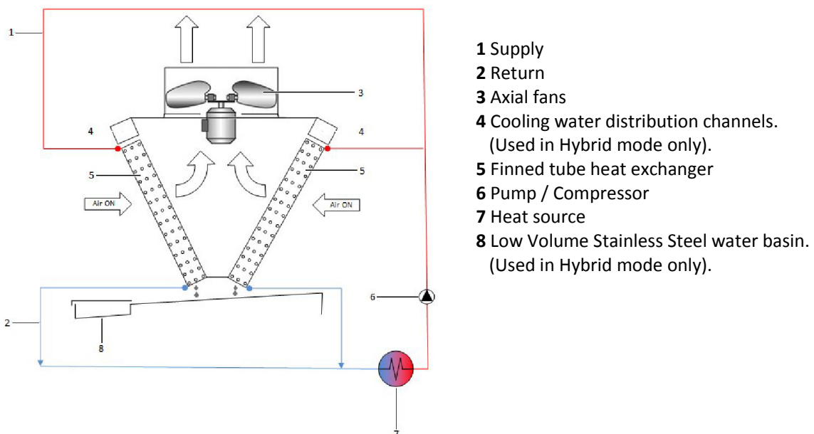
Image 2. Jaeggi Hybrid Dry Cooler/Condenser
