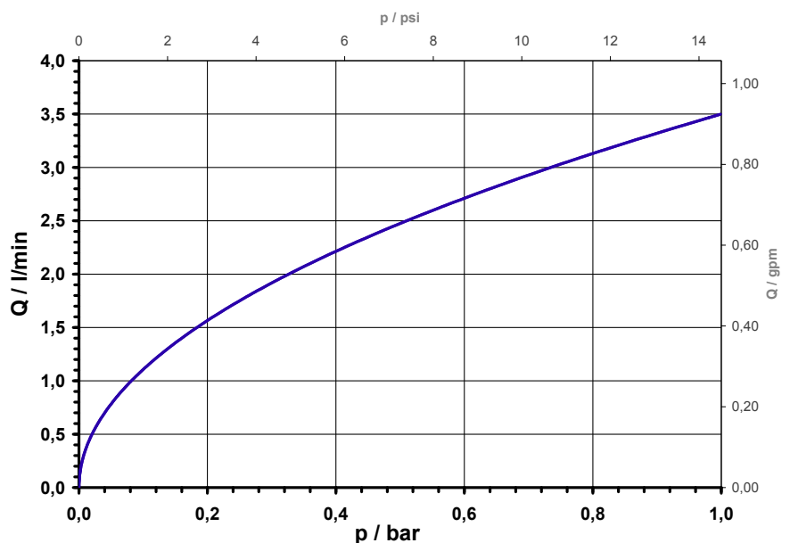
Typical performance curve Silicone tube 2,85x1,1; 60°Sh; length 30cm Medium: Water at 25°C; Free Outlet
