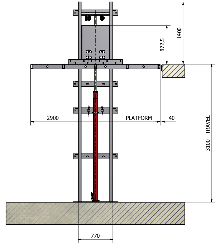
SECTION A-A UP POSITION
