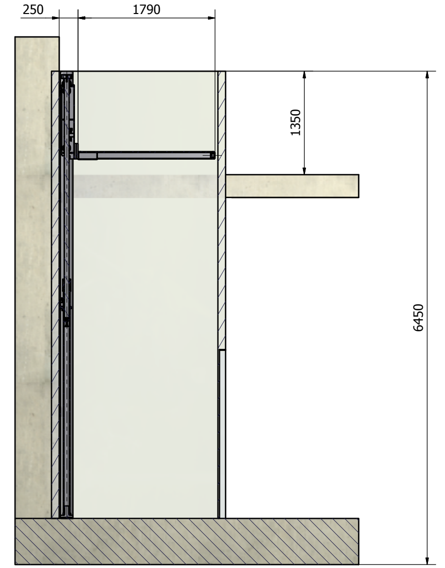
SECTION G-G
