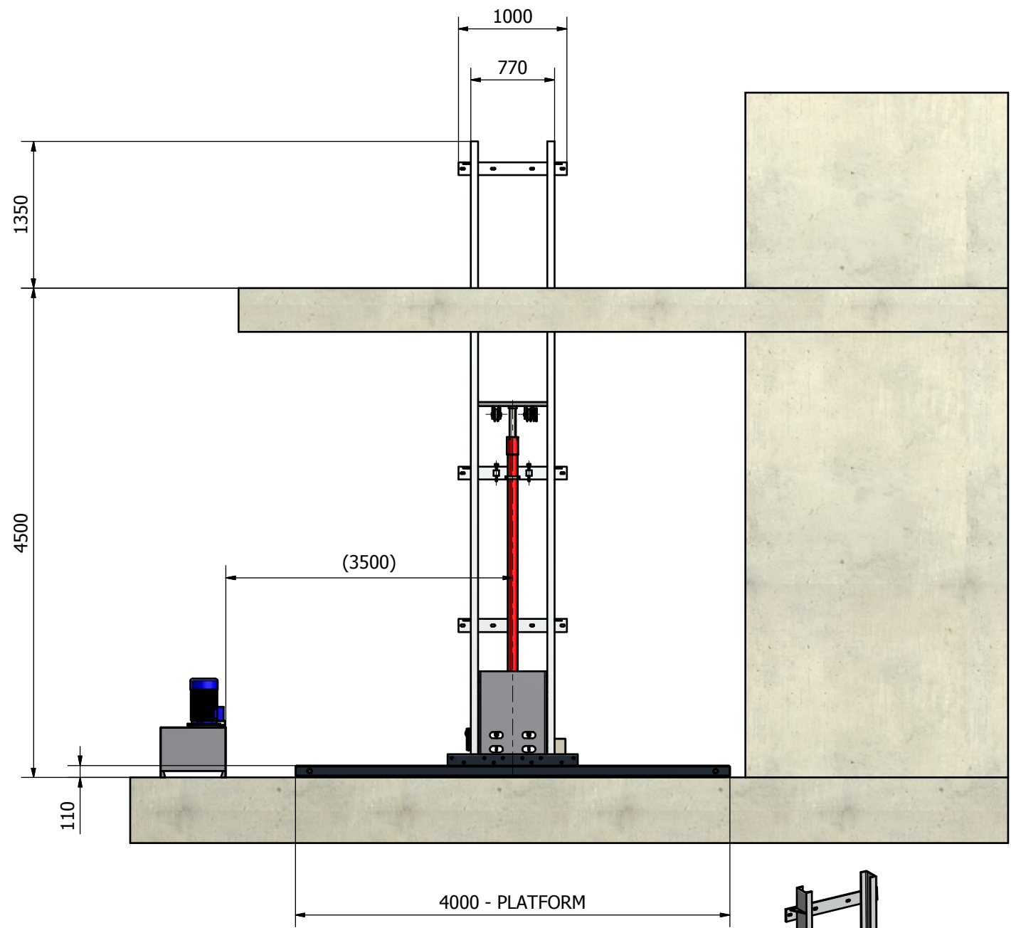
FRONT VIEW WITHOUT PROTECTIONS (LOWER POSITION)
