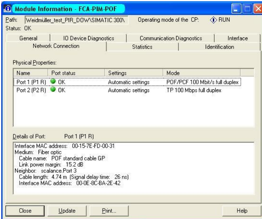
Figure 19 Step 7 device information
