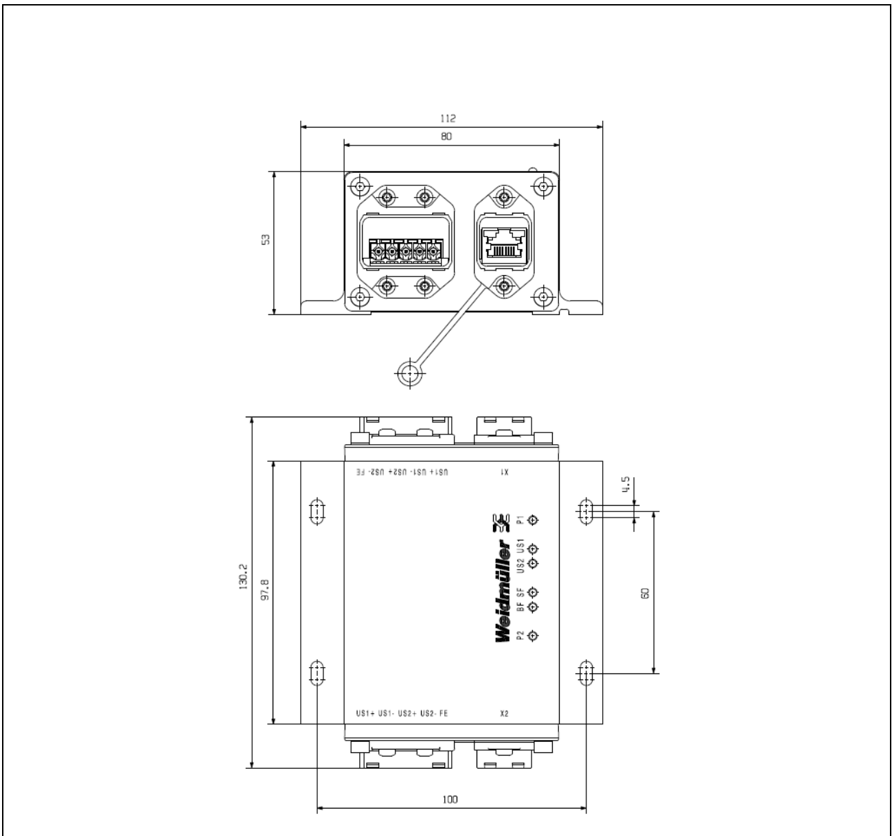
Figure 3 Mounting dimensions
