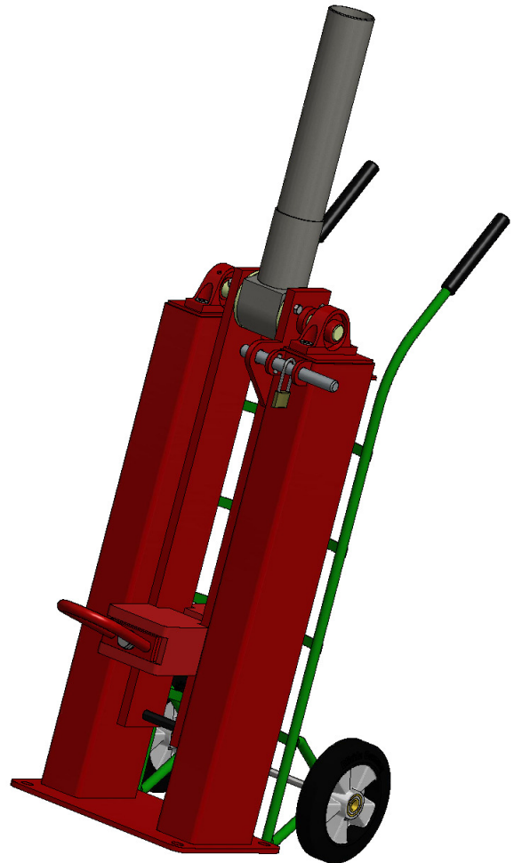
Figure 2A: Transporting
