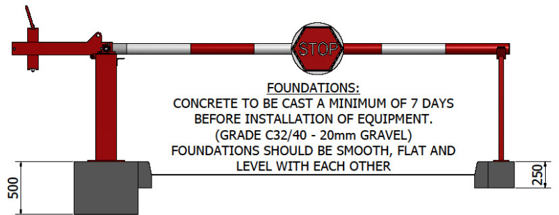
Figure 3 - Foundation Detail
