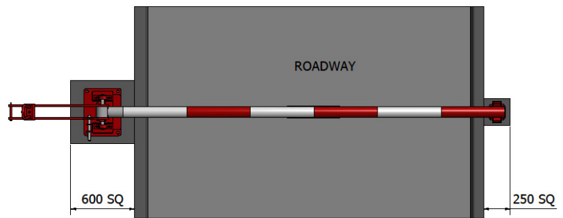
Figure 3 - Foundation Detail
