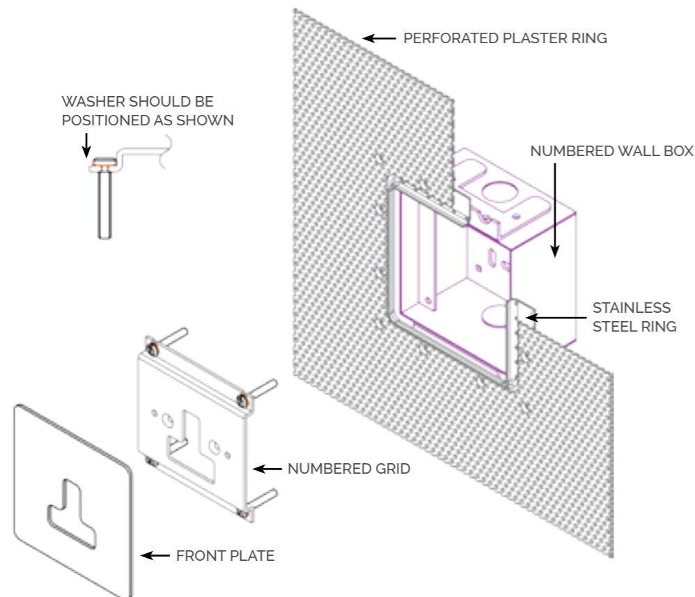
FIX WALL BOX AND PLASTER RING TO WALL
