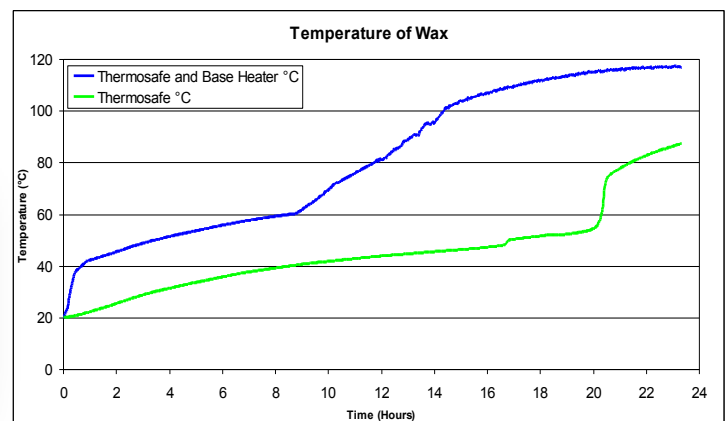
Temperature of Wax measured at hardest to heat location (base of drum in centre)
