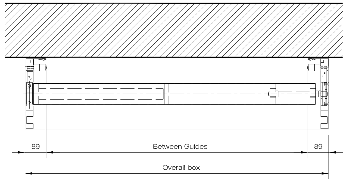
PLAN ON HEAD
