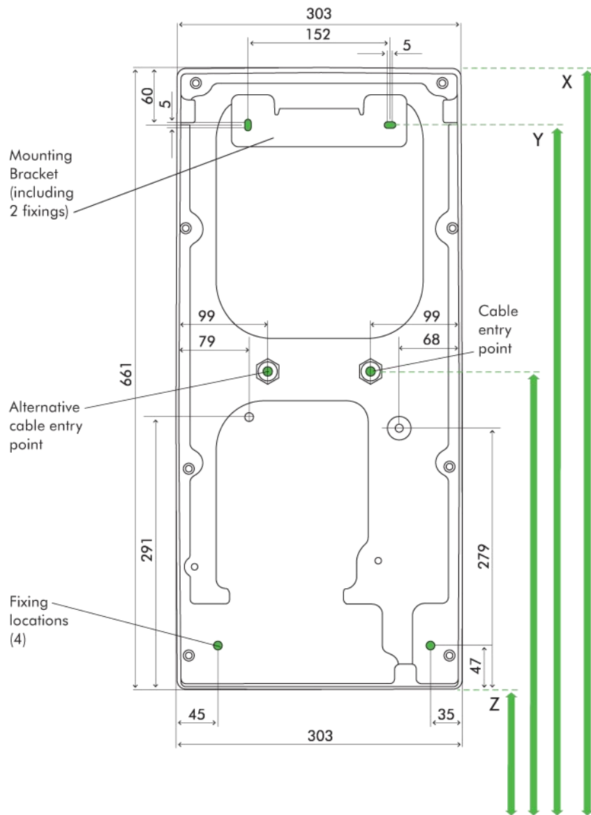
REAR ELEVATION
