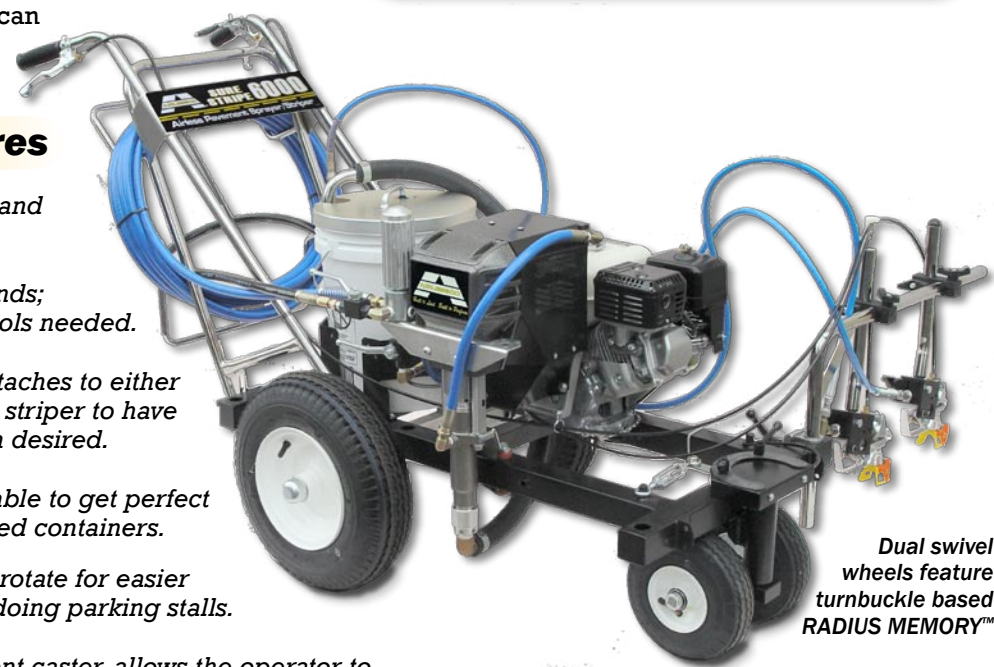
Model 6000 shown with dual guns & standard 50' of 3/4" hose
