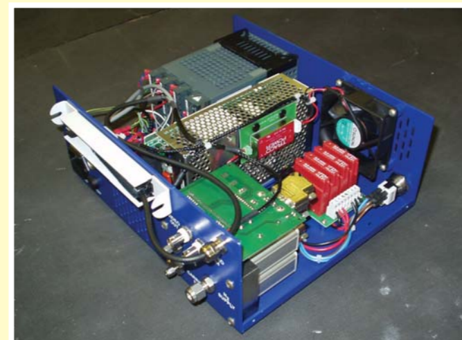
Fig 8 Enclosure assembly
