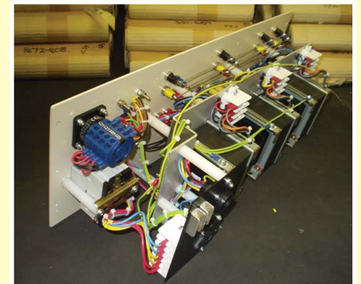
Fig 7 Control panel assembly
