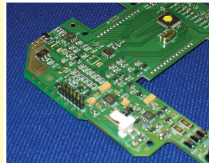
Fig 6 SM PCB assembly
