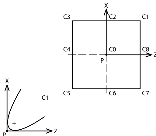
Definition of tool nose orientation
