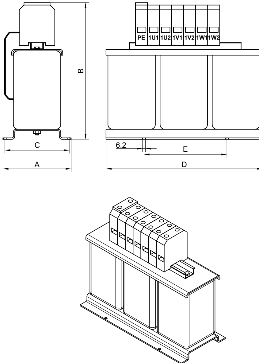
AGOIND001 and AGOIND002 - Overall Dimensions
