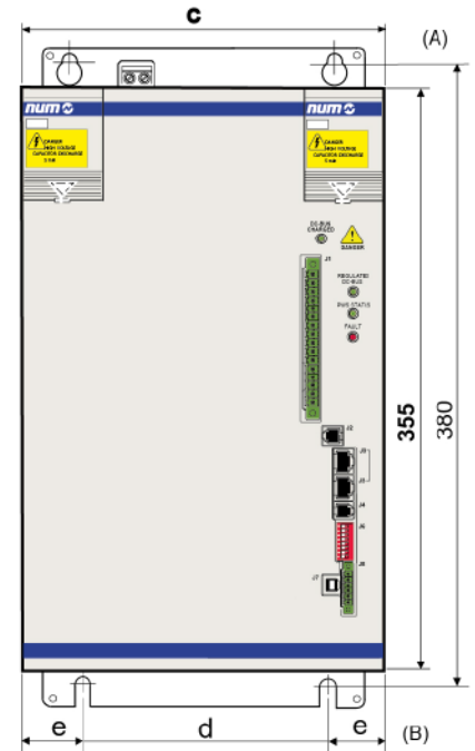
MDLL3 and MDLUX size 4 overall dimensions
