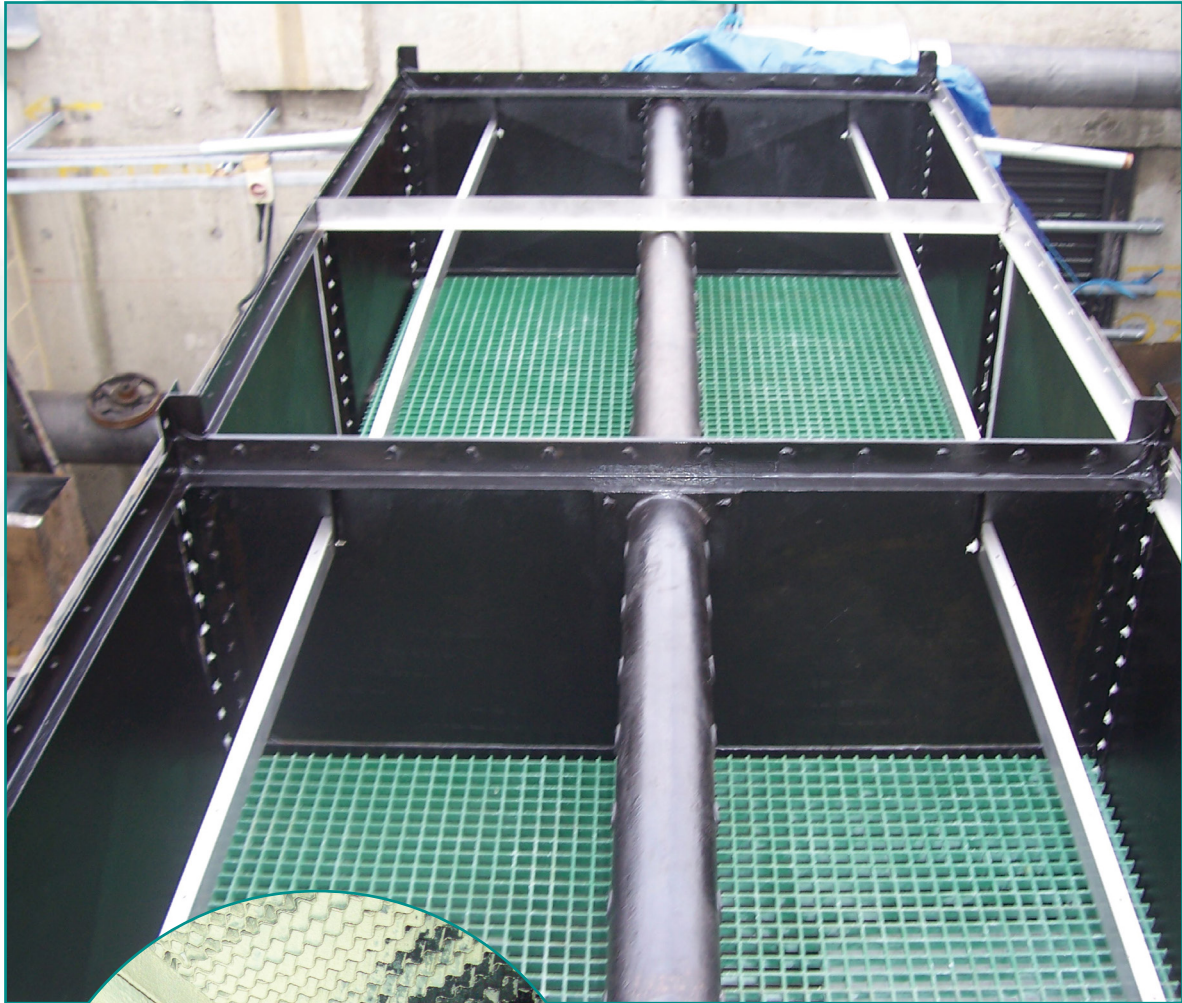
Safety Deck installed in newly refurbished cooling tower prior to fill pack installation
