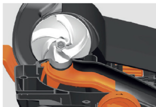
Efficient Impeller Technology Up to 17,000 rpm is driven by a timing belt that sucks in the dirt picked-up through to the filter bag.
