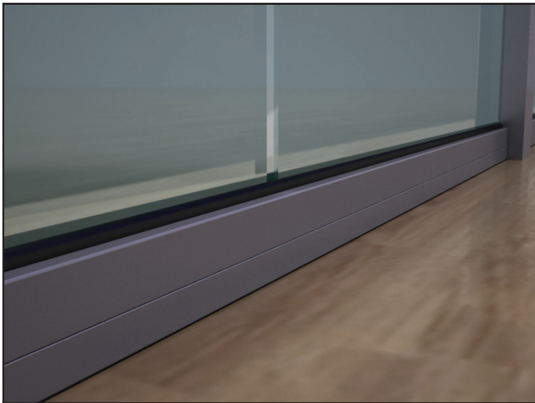
53 Using the 3mm glazing rubber provided glaze the bottom bead against the glass
