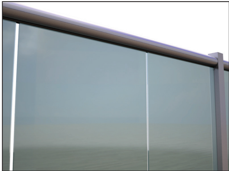
54 Using the 3mm glazing rubber provided glaze the handrail bead against the glass
