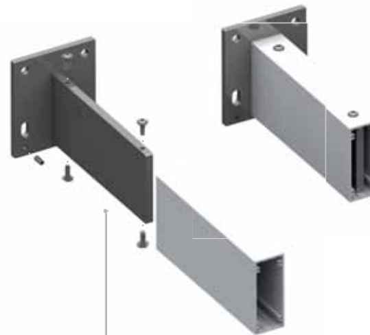
023104 SOPORTE A PARED PERFIL PORTANTE SUPPORT WALL SUPPORTING PROFILE SUPPORT MURAL PROFIL SUPPORT
