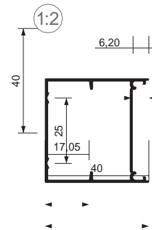
027394 TUBO ALUMINIO 40x40 AUTO-ROSCADO ALUMINIUM TUBE 40x40 SELF-TAPPING TUBE ALUMINIUM 40x40 AUTO-TARAUDAGE Escala Scale Echelle
