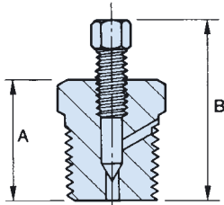
Vent Plug
