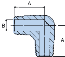
Male Elbow
