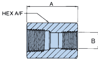
Hexagon Reducing Coupling NPT
