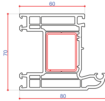
80mm Featured Sash 105175
