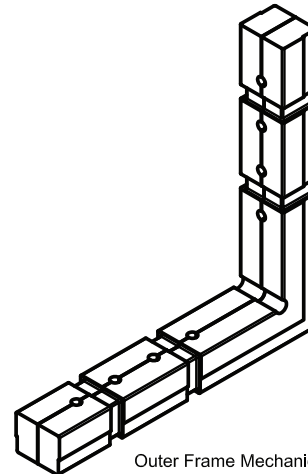
Moulded Gasket Corner 2 112448 #Available Black or White
