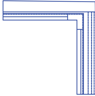
Moulded Gasket Corner 4 112454 #Available Black or White
