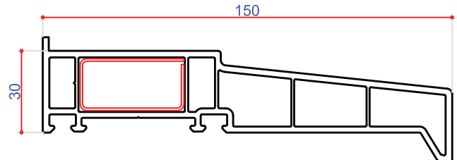
95mm Cill 110075 Steel U 38 x 19 113317 Steel Box 38 x 19 113245 End Cap 109075 Straight Cill Joint 109085 135° Cill Joint 109084 90° Cill Joint 109089
