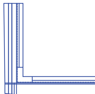
Moulded Gasket Corner 2 112448 #Available Black or White
