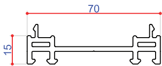
15mm Frame Extension 114028
