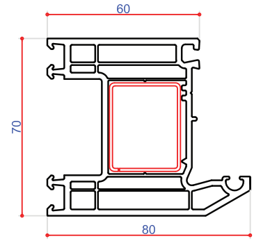
80mm Chamfered sash 105176
