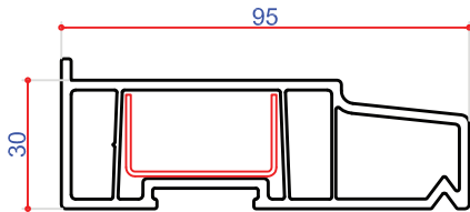
95mm Cill 110074 Steel U Channel 35 x 19mm 113377 End Cap 109074
