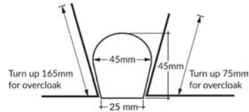
F. Standard wood cored roll with splash lap
