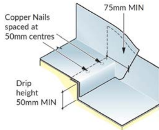
D. Tapered gutter drip without splash laps
