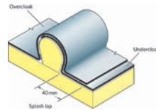
G. Roll drip intersections for wide gutters
