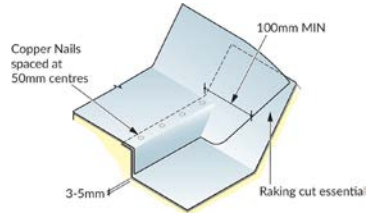
D. Tapered gutter drip without splash laps
