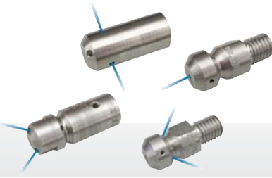
Nozzles with multiple bores for heat exchanger bundle tube internal cleaning
