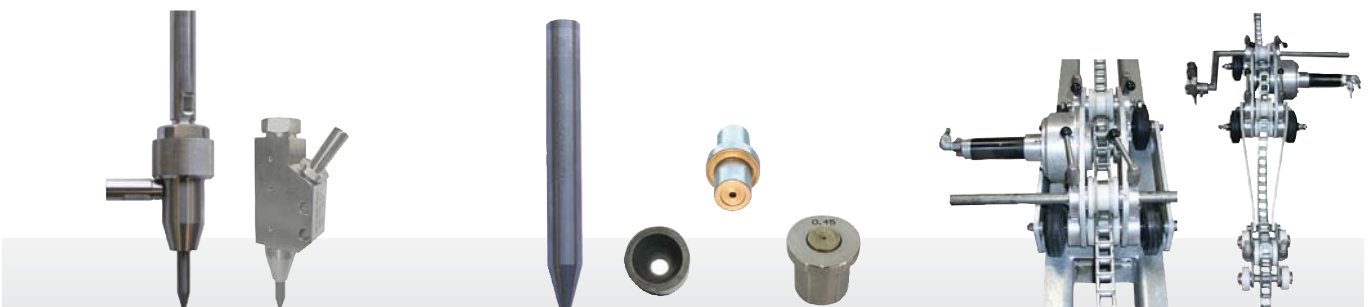
A water jet entrains the abrasive inside the cutting head housing
