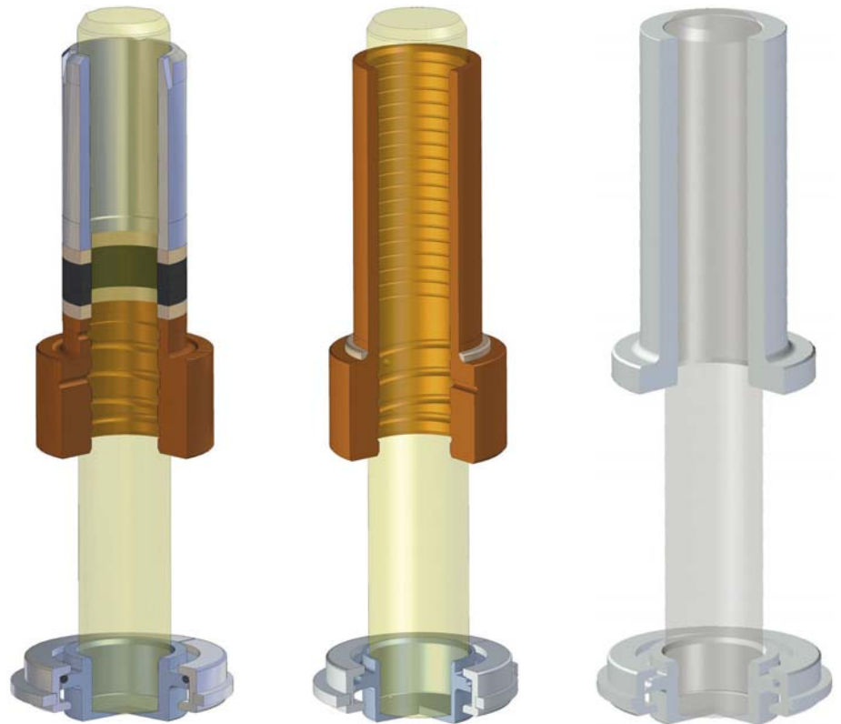
Packed sealing up to 1600 bar
