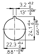
Without interlock M = 17,7 C = 5 .70 .20
