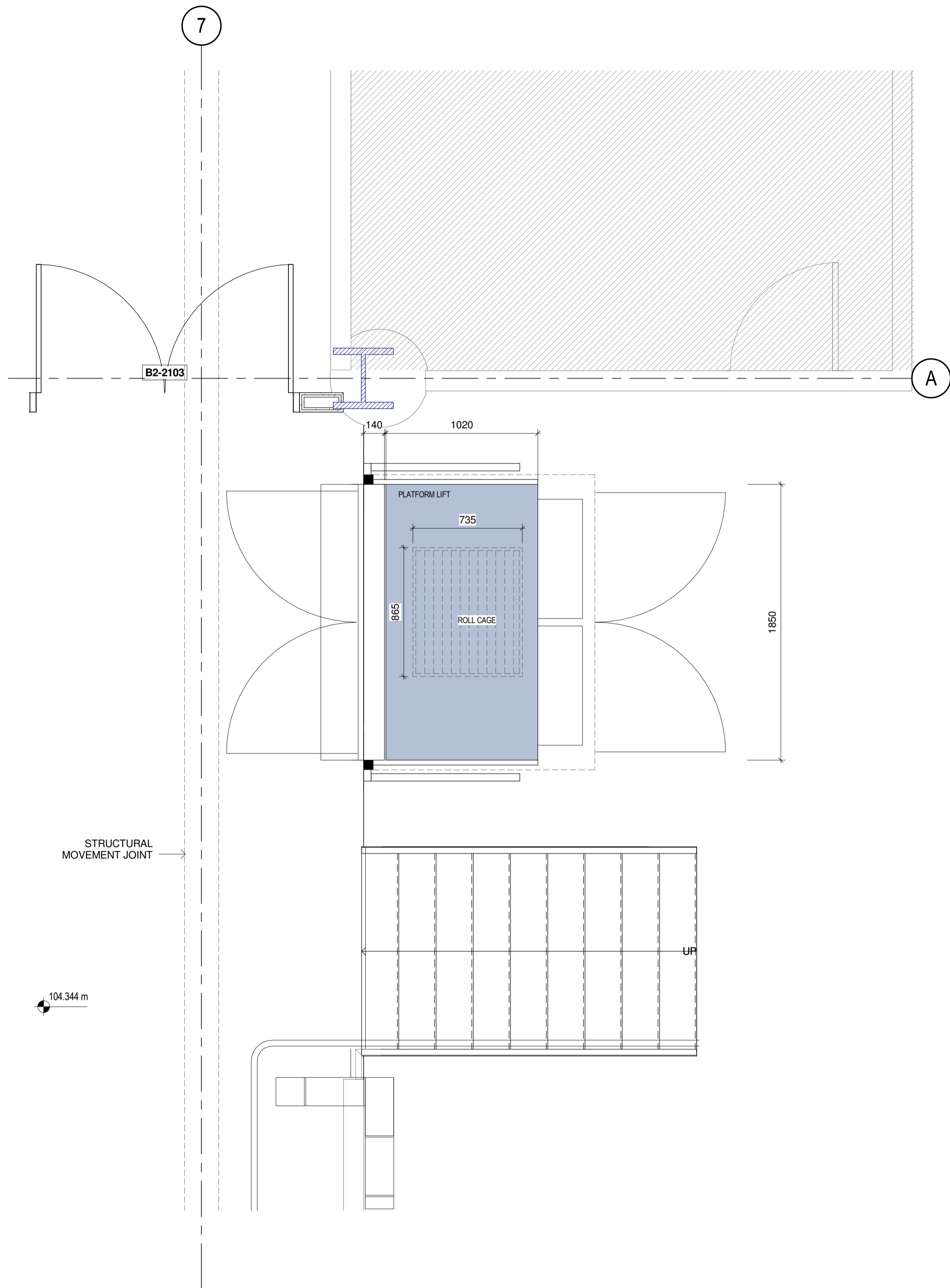
1 GA Mezzanine - Platform Lift 1 : 20
