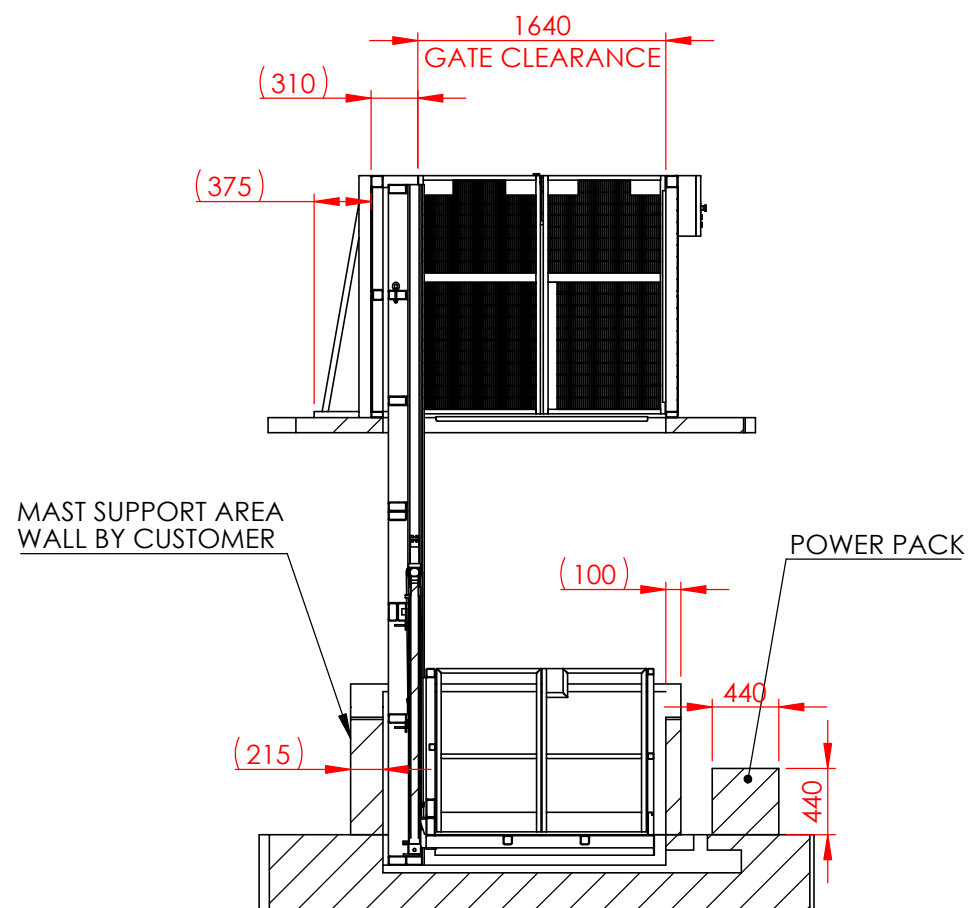
SECTION C-C
