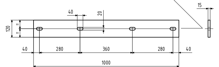
FIXING PLATE DETAIL
