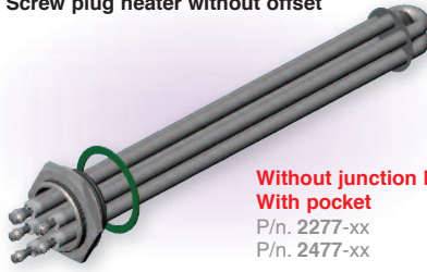
Screw plug heater without offset
