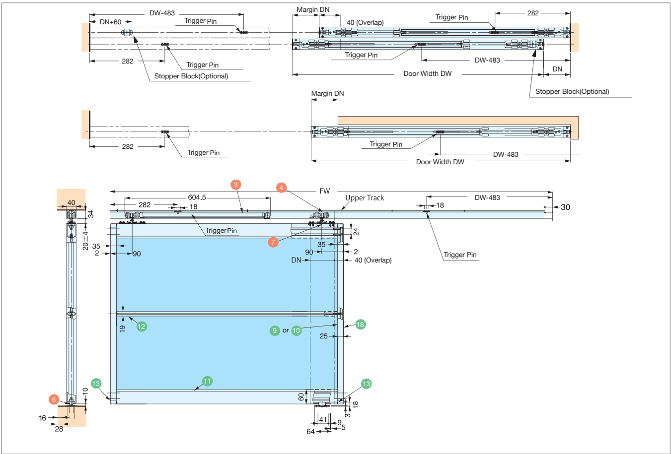
C FD80-AF / Surface Mount Roller / Two-Way Soft Close
