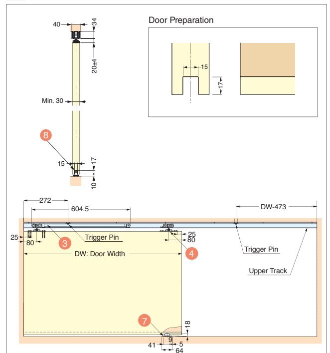
d FD80 / Surface Mount Roller / Standard Sliding
