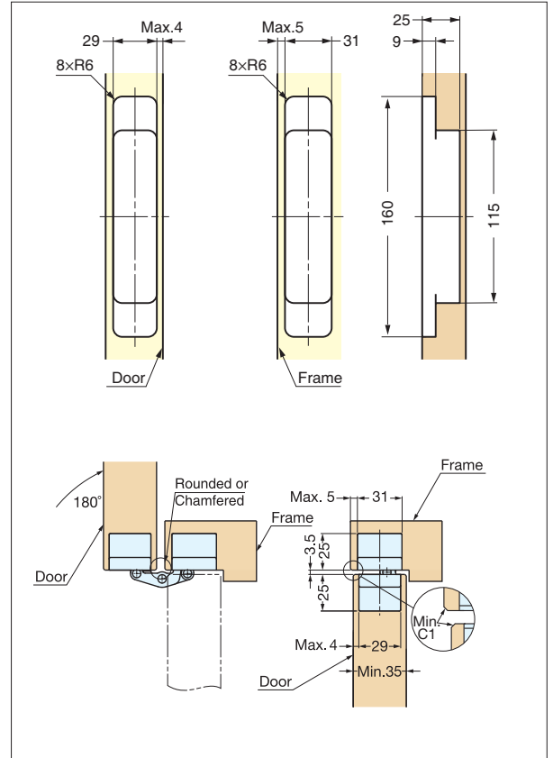
Bore Dimensions
