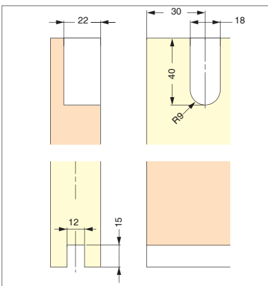
c FD30 / Recessed Mount Roller / Standard Sliding
