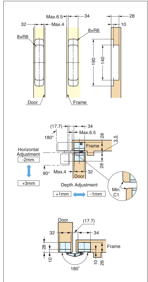
Bore Dimensions
