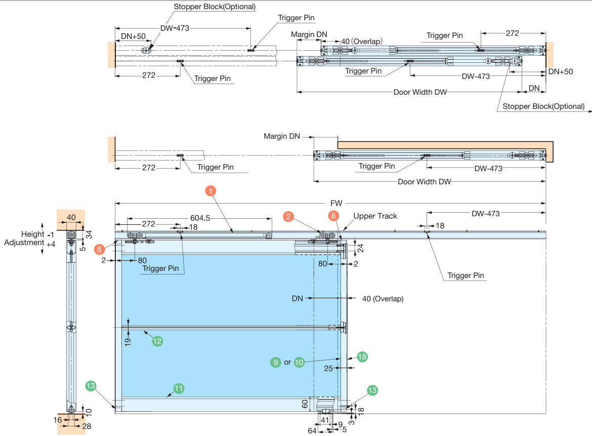
a FD80-AF / Recessed Mount Roller / Two-Way Soft Close
