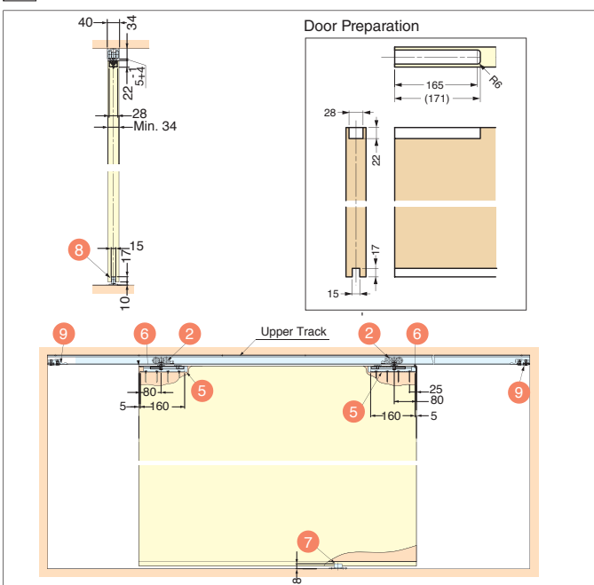
b FD80 / Recessed Mount Roller / Standard Sliding
