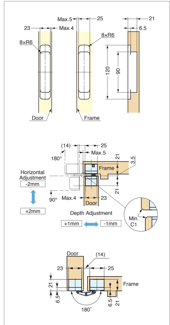
Bore Dimensions
