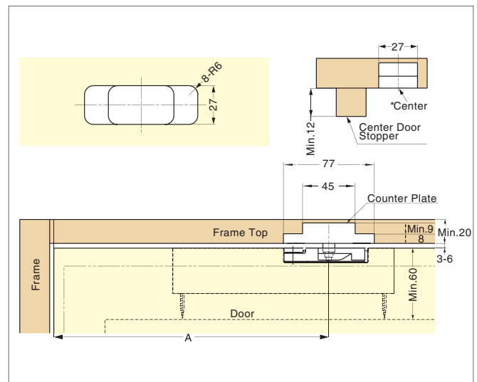
Bore Dimensions (Frame)
