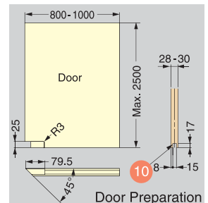
Door Preparation
