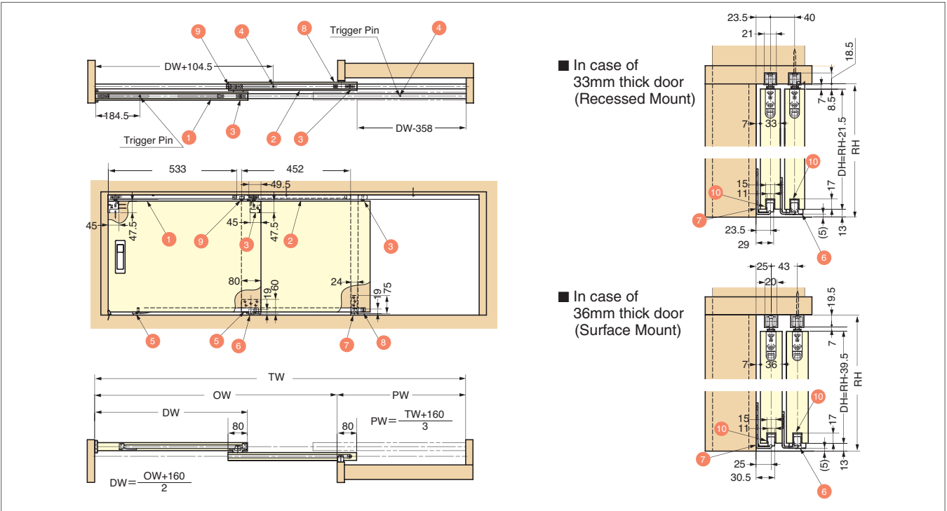
b FD30 / Synchronized Sliding / 3 doors
