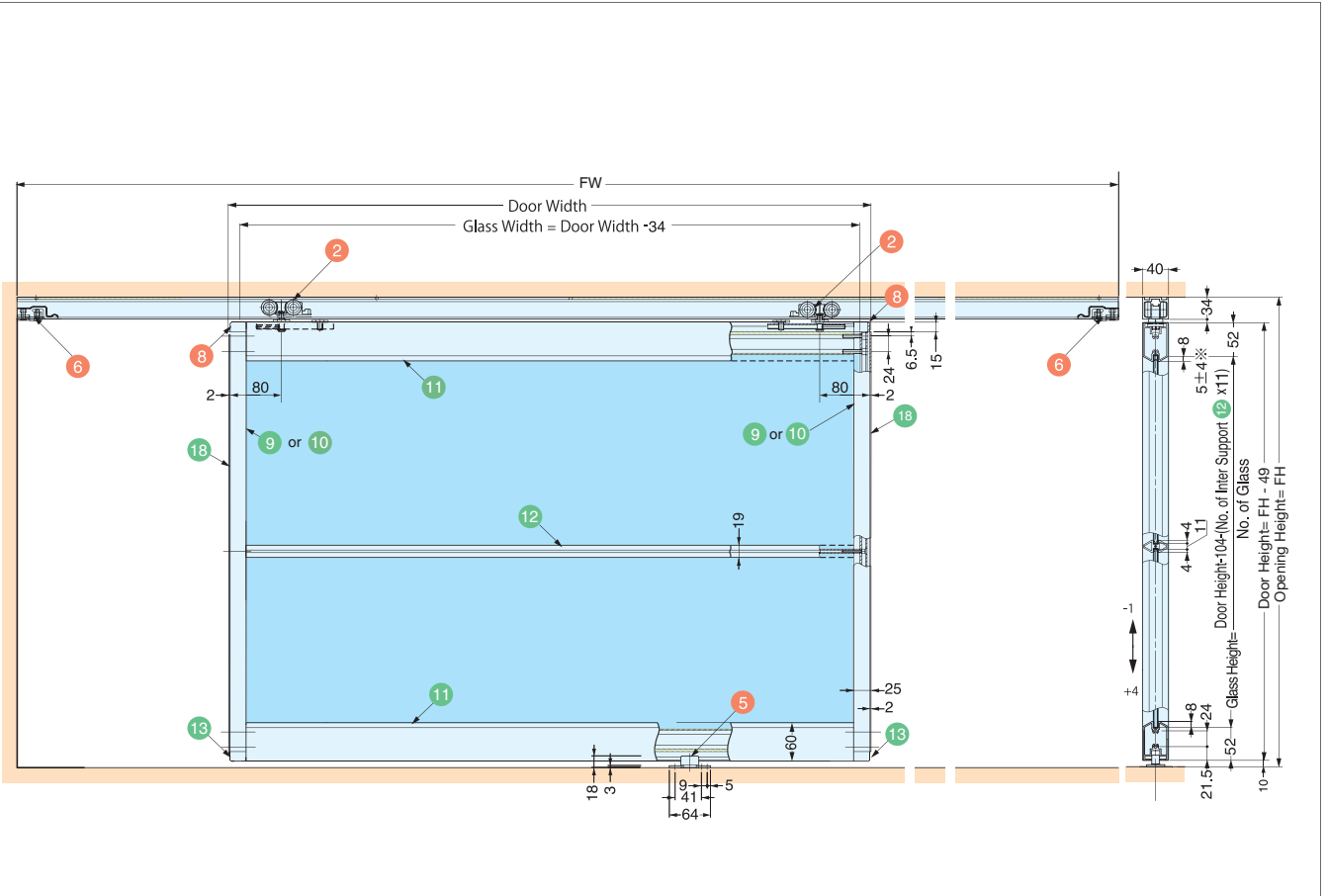
b FD80-AF / Recessed Mount Roller / Standard Sliding
