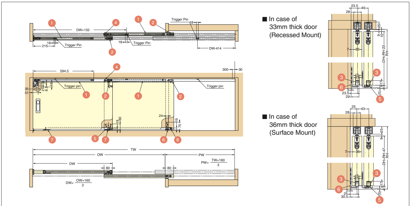
a FD50 / Synchronized Sliding / 2 doors
