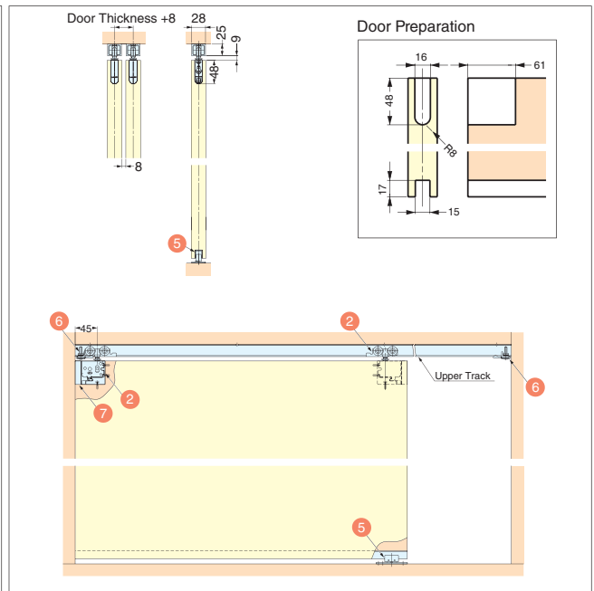
d FD50 / Surface Mount Roller / Standard Sliding
