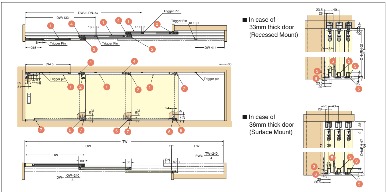
b FD50 / Synchronized Sliding / 3 doors
