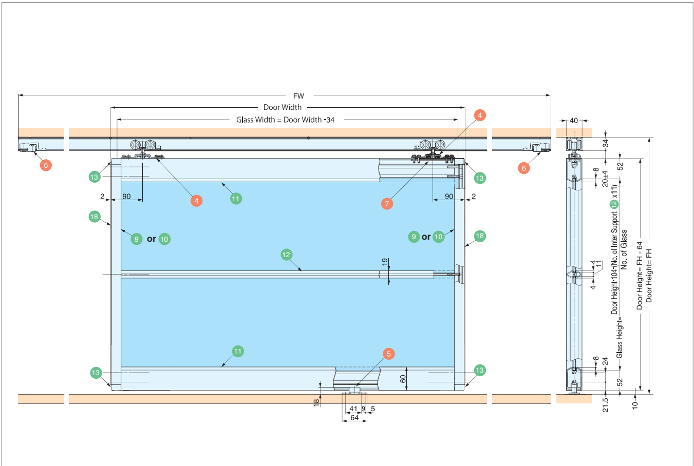
d FD80-AF / Surface Mount Roller / Standard Sliding
