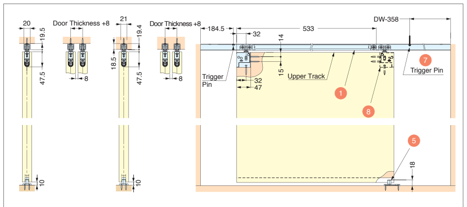
b FD30 / Recessed Mount Roller / One-Way Soft Close
