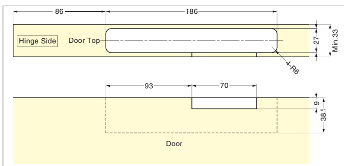
Bore Dimensions (Door)
