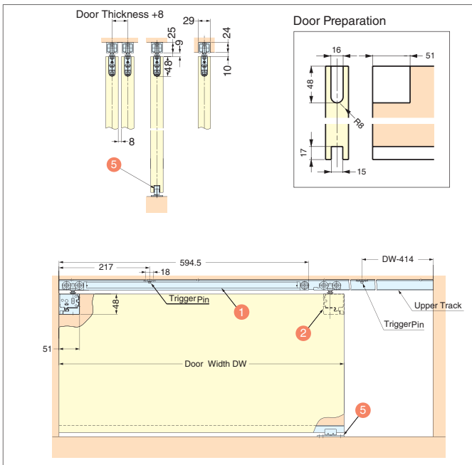
c FD50 / Surface Mount Roller / Two-Way Soft Close
