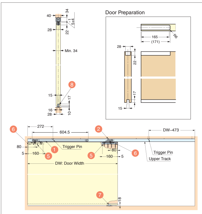
b FD80 / Recessed Mount Roller / Standard Sliding
