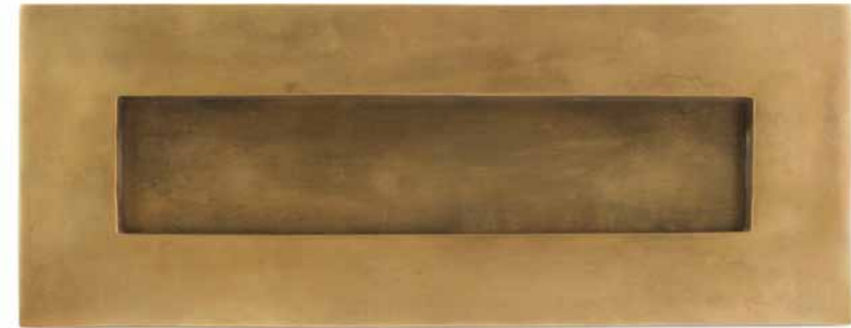
765 / 766 Letter Plate 765 (M) Overall 264 x 103mm, opening 200 x 44, fixing centres 233mm 766 (L) Overall 352 x 104mm, opening 244 x 47, fixing centres 302mm Available in all finishes
