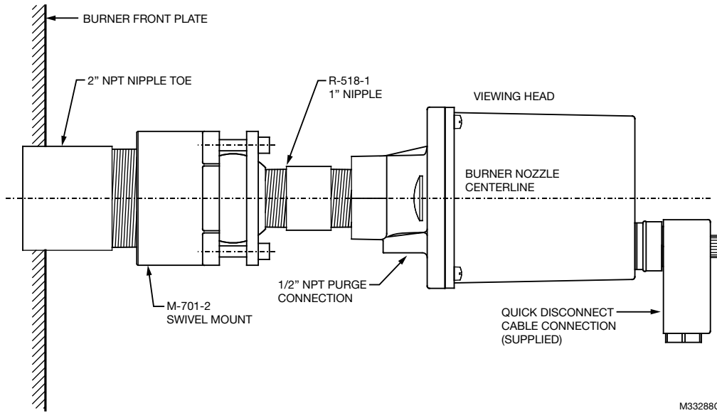
Fig. 7. Viewing head mounting example.
