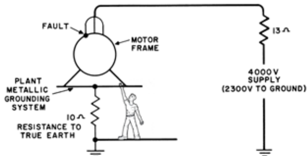
Fig. 7: Example of an electrical circuit with too high an earth resistance
