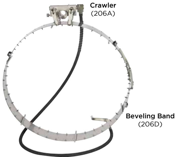
206D 12"-146"+ 206A-9 Beveling Crawler w/9' Shaft
