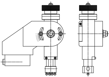
TOOLBOX FOR INSIDE BEVEL AND ID BORING UP TO 100 MM DEPTH.
